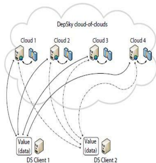
Figure 2: DepSky Architecture [8].
