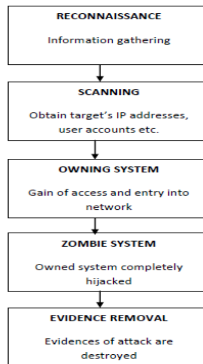
Fig. 2 Hacking Phases
