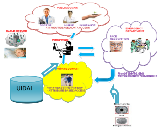
System Architecture
