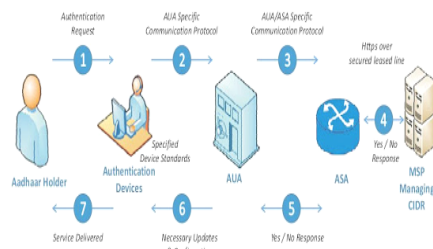
UIDAI Architecture
