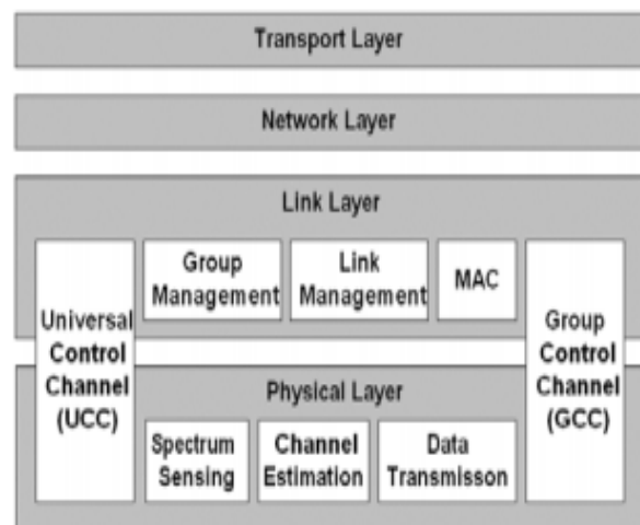
Fig. 2: General ISO/OSI Model for Cognitive Radio [24]
