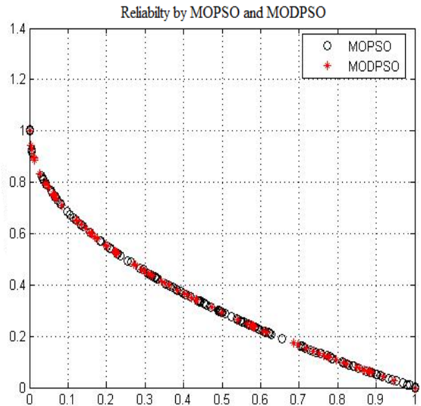
Fig. 8 Reliability comparison by MOPSO and MODPSO
