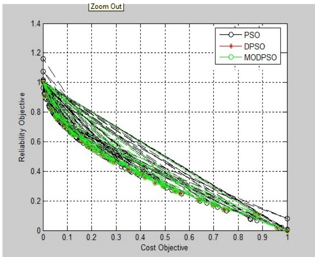
Fig. 9 Results for 50 iterations
