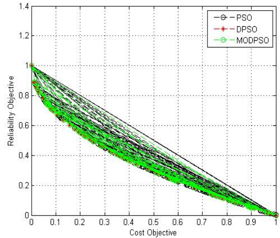
Fig. 12 Results for 200 iterations
