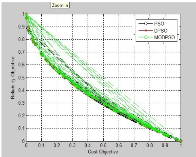
Fig. 10 Results for 100 iterations
